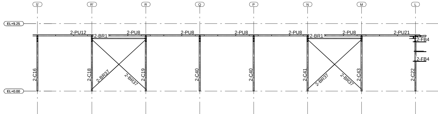
SECTION GRID X2
