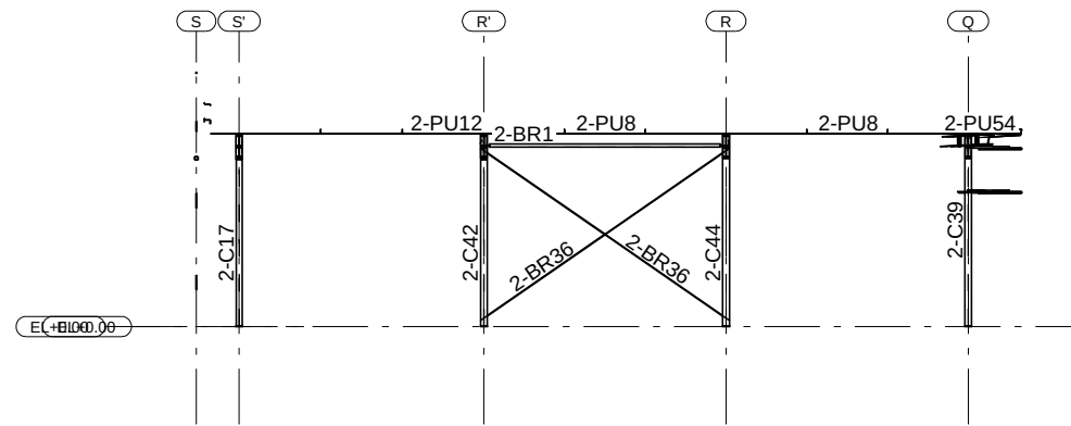
SECTION GRID X1
